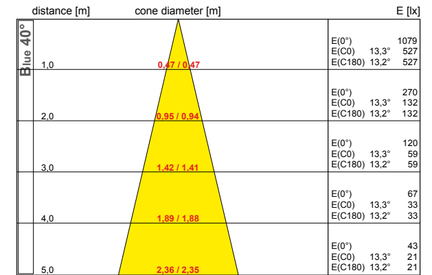
half value angle C0-180 : 26,6° C90-270 : 26,4° 24xLED, total flux: 528,0 lm, LOR: 60%
